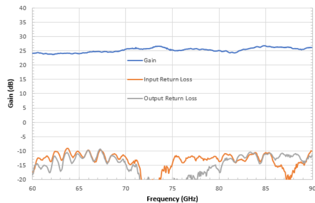
Gain and Return Loss vs. Frequency Bias: +8 V DC /260 mA
