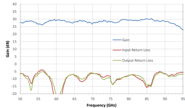
Gain and Return Loss vs. Frequency Bias: +8 V DC /260 mA
