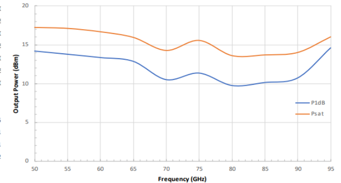
Typical Output Power vs. Frequency Bias: +8 V DC /270 mA
